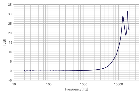
Fig.1 CRY3717 Coupler + CRY3102 Microphone + CRY508C Preamplifier Frequency Response
