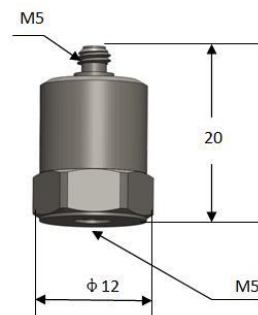
Fig.2 CRY431 Accelerometer Drawings
