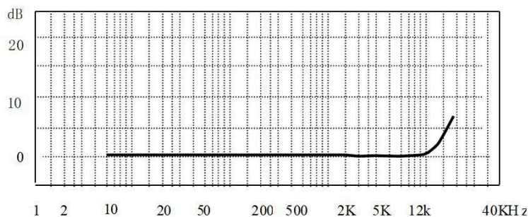
Fig.1 CRY431 Accelerometer Typical Frequency Response
