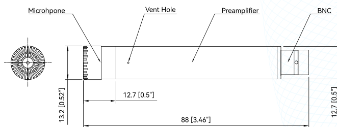
Fig.2 CRY3202-S01 Microphone Set Drawings
